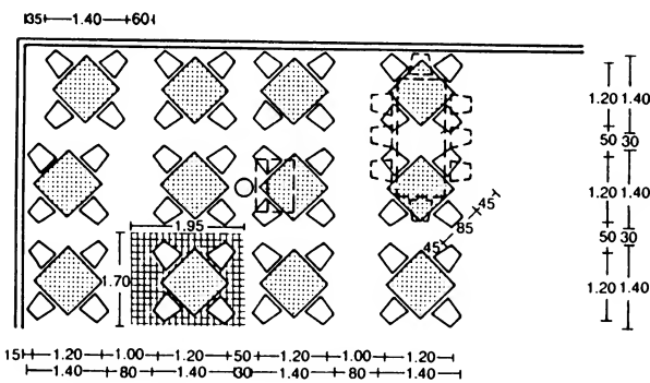
④ Diagonal table arrangement
